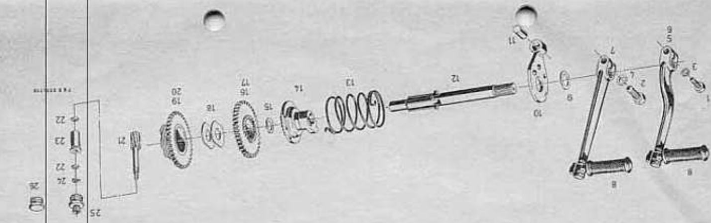
Kickstarter, Tachometer-Antrieb
